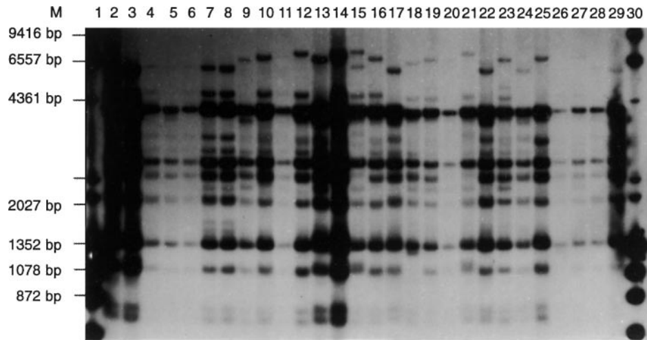
Fig. 3 Southern-blotting analysis in the genus Phaseolus using an EcoRI digest of total DNA and probed by the purified cpDNA. Lane 1 Molecular size marker (M) lane 2 P. bolivianus , lane 3 P. pachyrrhizoides , lane 4 P. augusti , lane 5 P. polystachyus , lanes 6–8 P. lunatus (G25225, G25583, G25294 C), lane 9 P. microcarpus , Lane 10 P. leptostachyus , lane 11 P. filiformis , lane 12 P. vulgaris , lane 13 P. filiformis , lane 14 P. vulgaris , lane 15 P. oligospermus , lane 16 P. angustissimus , lane 17 P. maculatus , lane 18 P. hintonii , lane 19 P. pedicellatus , lane 20 P. microcarpus , lane 21 P. oligospermus , lane 22 P. salicifolius , lane 23 P. grayanus , lane 24 P. marechalii , lane 25 P. coccineus , lane 26 P. hintonii , lane 27 P. grayanus , lane 28 P. marechalii , lane 29 P. maculatus
